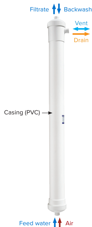
Port connections
